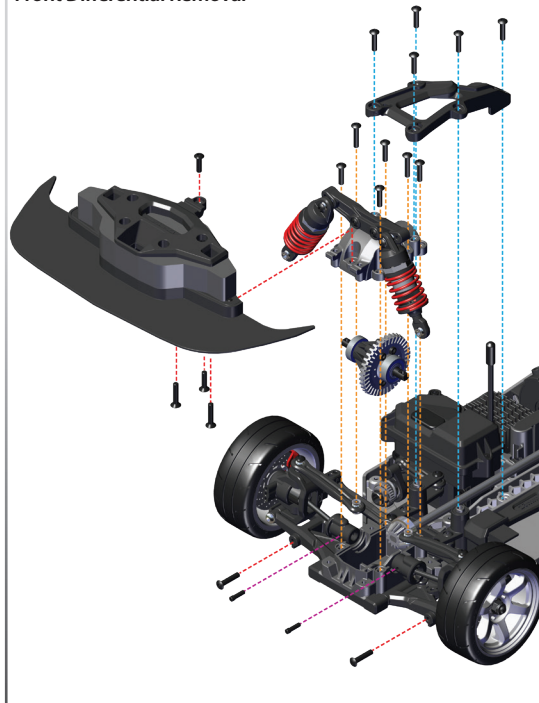
Front Differential Removal
