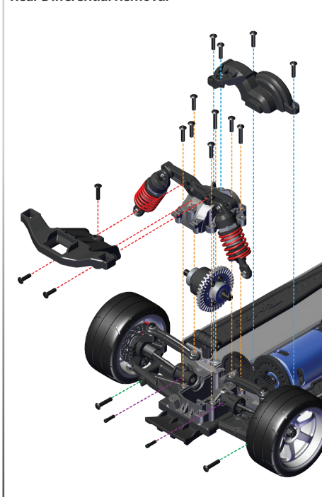
Rear Differential Removal
